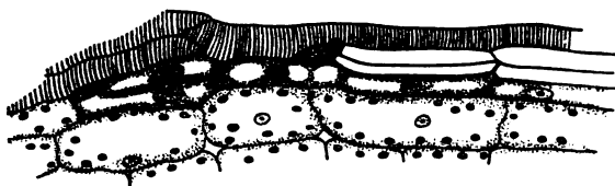
FIG. 9. — A leaf veinlet, in longitudinal section, of Fuchsia globosa ; greatly magnified. Above are the tracheids, and below are sieve tubes and associated cells, but the sheath cells do not show in the drawing. (From Haberlandt's Physiological Plant Anatomy .)
